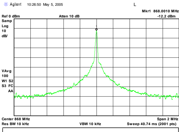
At 868 MHz
