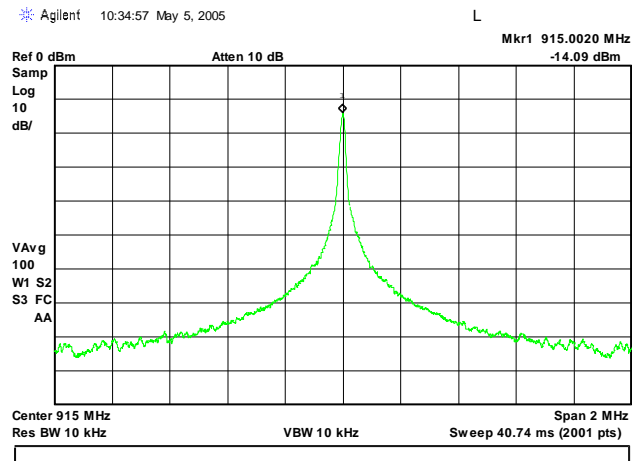
At 915 MHz
