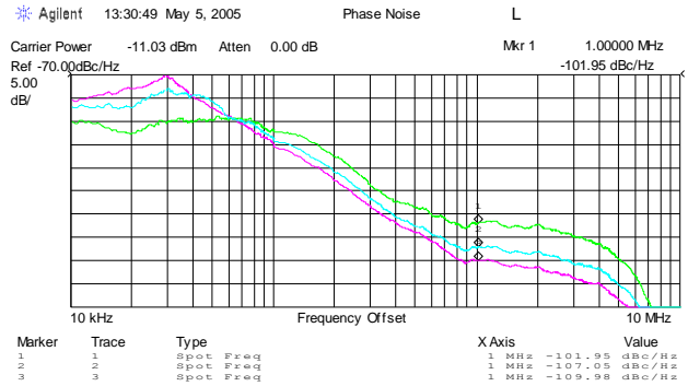
100, 50, 33% Charge pump current settings (Ref. level: -70 dBc/Hz, 5 dB/div)
