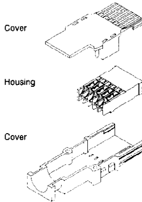
10 Positions, Unshielded
