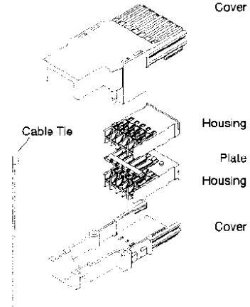
20 Positions, Unshielded
