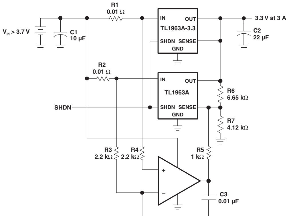
Figure 31. Paralleling Regulators for Higher Output Current
