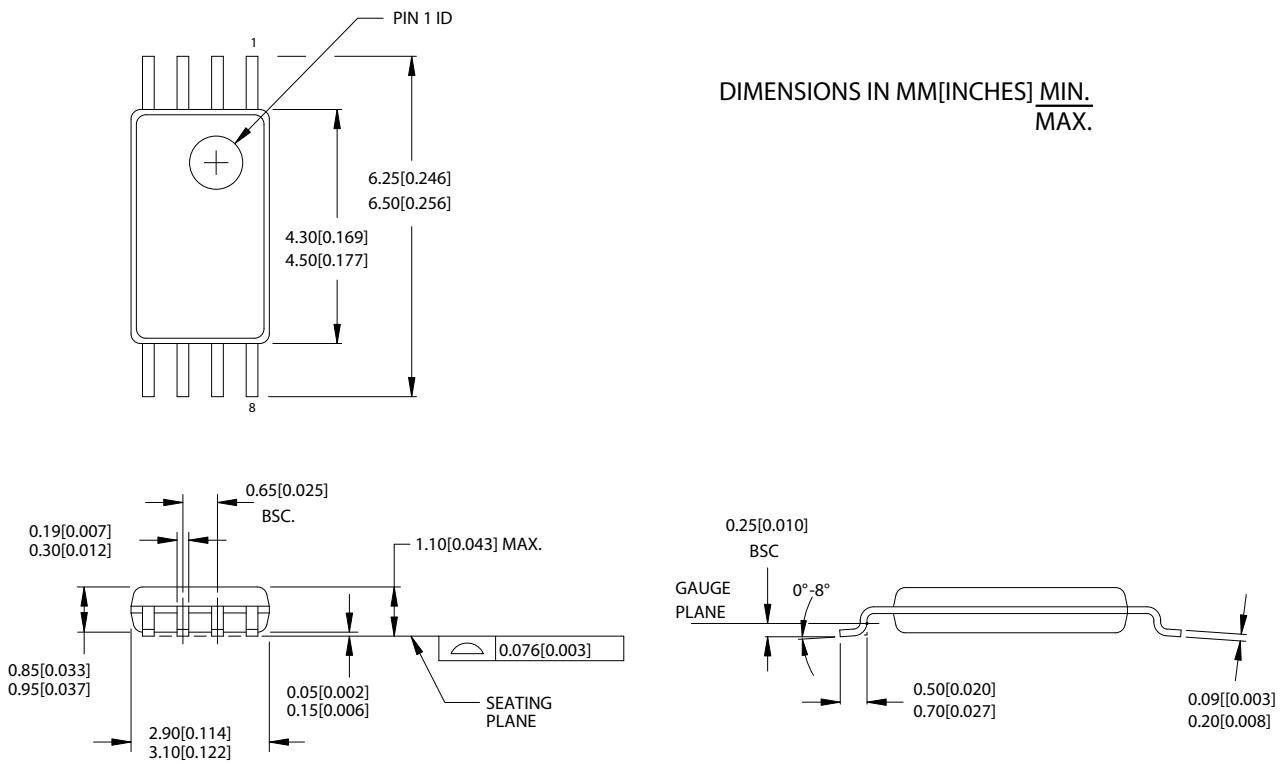
Figure 11. 8-Pin Thin Shrunken Small Outline Package (4.40 MM Body) Z8
