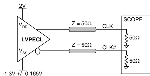
Figure 2. 3.3V Output Load AC Test Circuit
