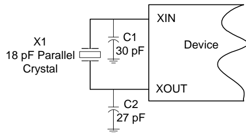
Figure 10. Crystal Input Interface
