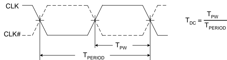
Figure 7. Output Duty Cycle
