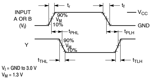
Figure 3. Switching Waveforms
