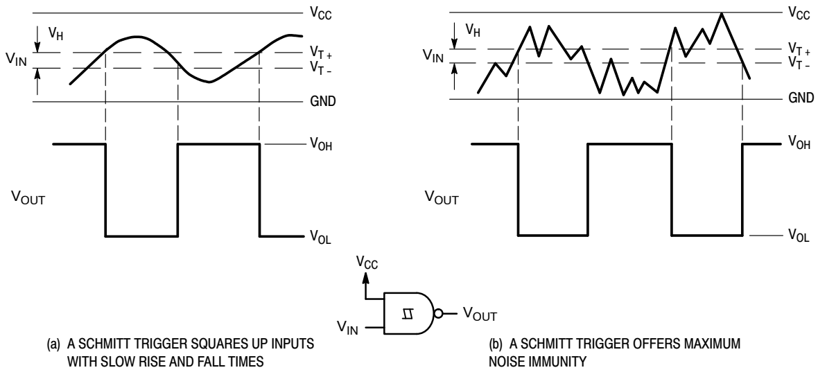
Figure 5. Typical Schmitt-Trigger Applications
