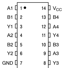
Figure 1. Pin Assignment
