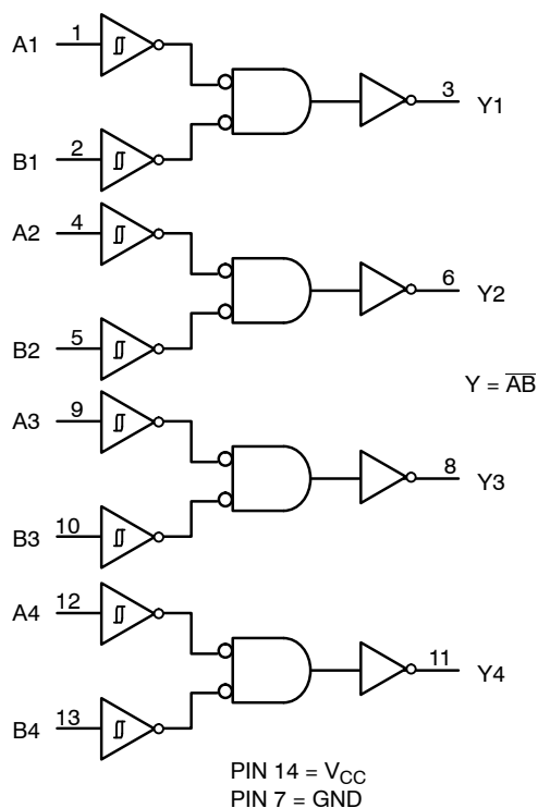
Figure 2. Logic Diagram
