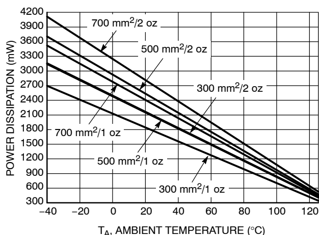
Figure 7. Power Dissipation vs. Ambient Temperature @ T_J = 150^{\circ}\text{C}
