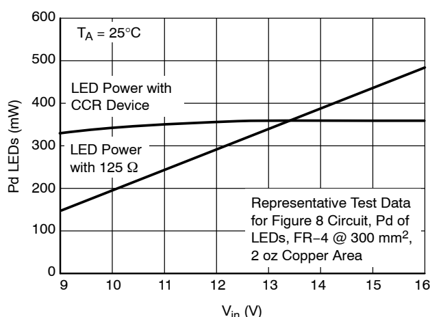
Figure 11. LED Power
