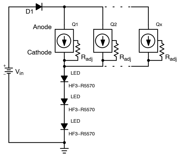
Figure 9. Typical Application Circuit (90 mA each LED String)
