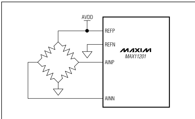
Figure 7. Resistive Bridge Measurement Circuit
