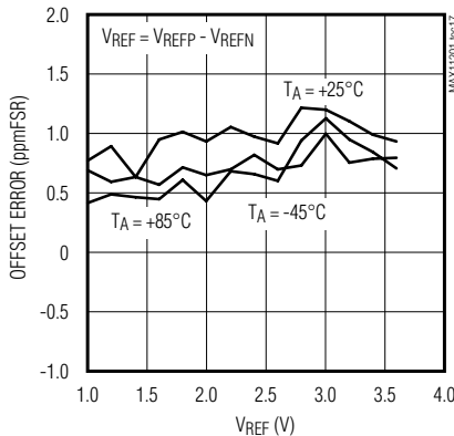
OFFSET ERROR vs. VREF
