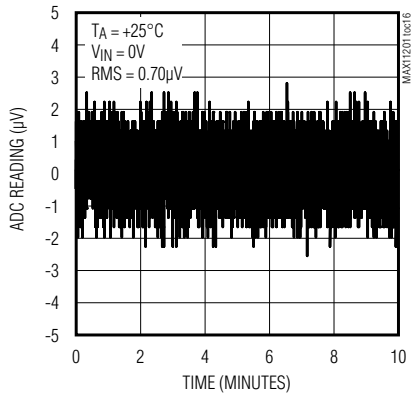
LONG-TERM ADC READINGS (MAX11201B)
