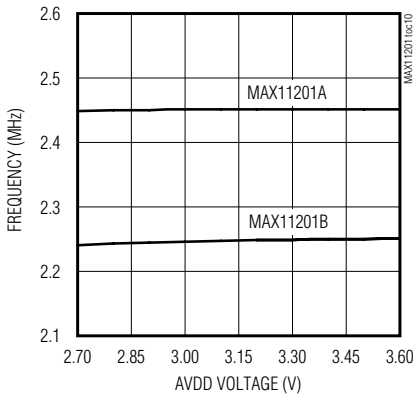
INTERNAL OSCILLATOR FREQUENCY vs. AVDD VOLTAGE
