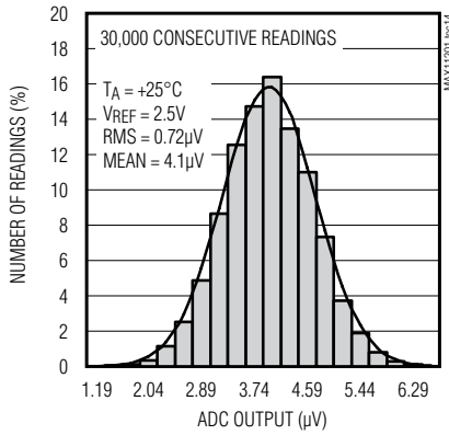
NOISE HISTOGRAM (MAX11201B, 13.75sps)
