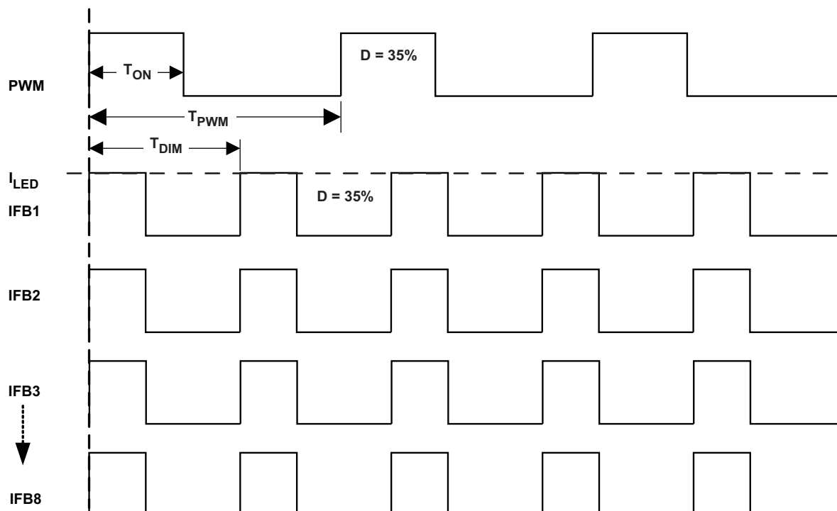
Figure 15. No Delay PWM Dimming Timing Diagram
