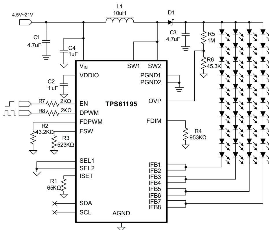
Figure 24. Typical Application Circuit for 4 Strings 40mA LED
