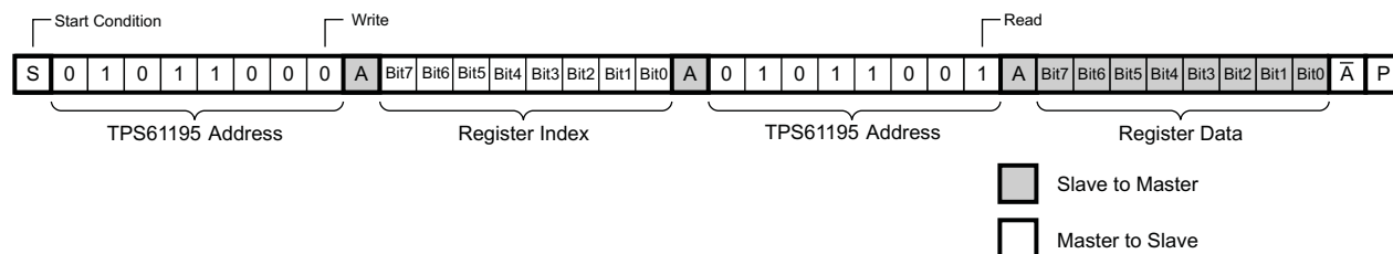
Figure 19. TPS61195 SMBus Read Byte Protocol
