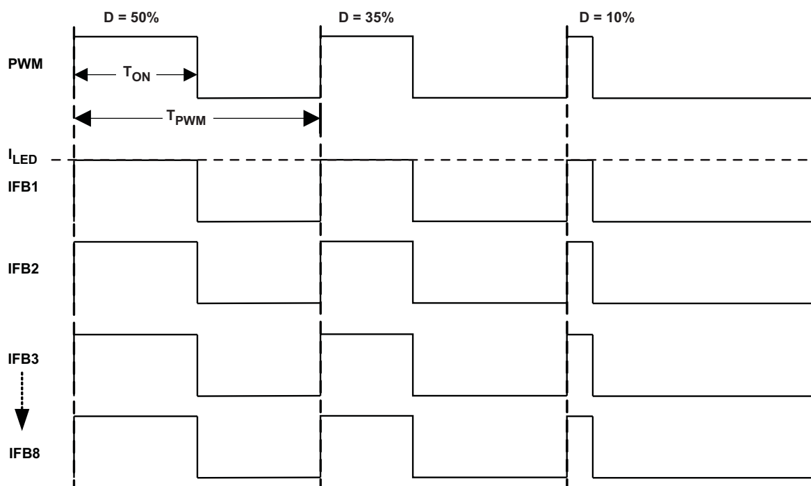
Figure 16. Direct PWM Dimming Timing Diagram
