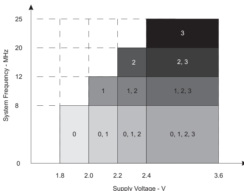
Figure 5-1. Maximum System Frequency
