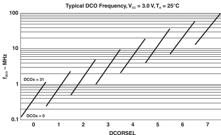
Figure 5-10. Typical DCO frequency
