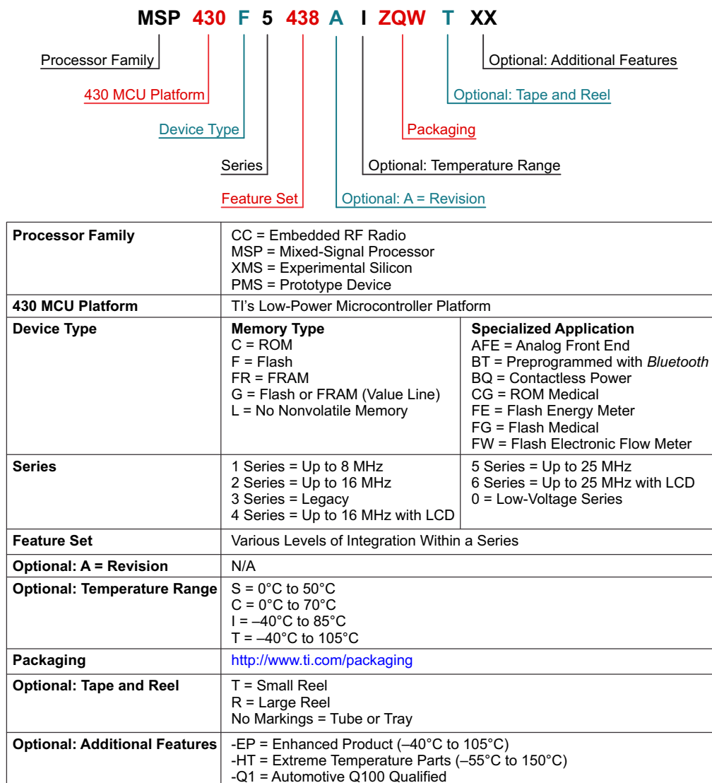
Figure 7-1. Device Nomenclature
