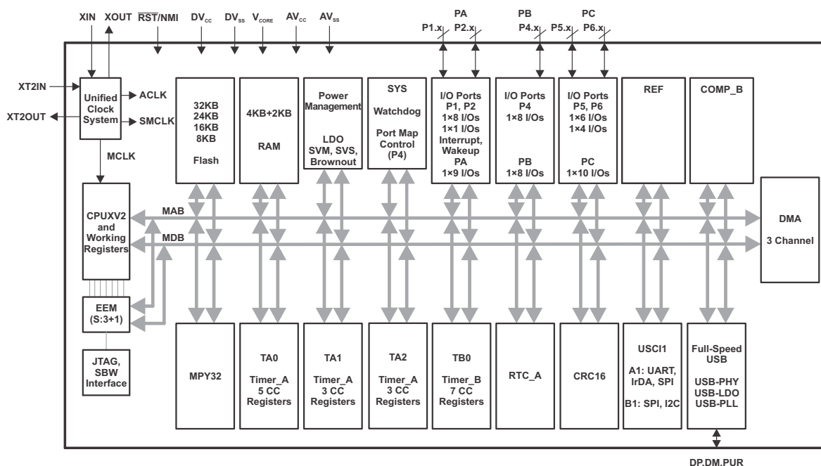
Figure 1-4. Functional Block Diagram – MSP430F5503IRGZ, MSP430F5502IRGZ, MSP430F5501IRGZ, MSP430F5500IRGZ
