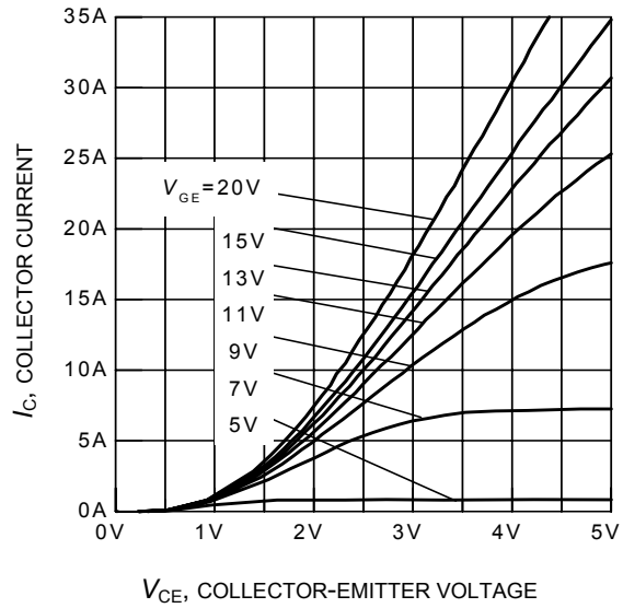
Figure 6. Typical output characteristics ( T_j = 150^\circ\text{C} )
