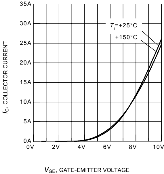
Figure 7. Typical transfer characteristics ( V_{CE} = 10\text{V} )
