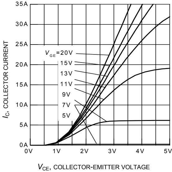
Figure 5. Typical output characteristics ( T_j = 25^\circ\text{C} )
