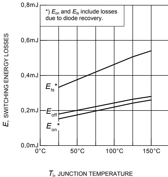
T_j , JUNCTION TEMPERATURE Figure 15. Typical switching energy losses as a function of junction temperature (inductive load, V_{CE} = 400\text{V} , V_{GE} = 0/+15\text{V} , I_C = 10\text{A} , R_G = 25\Omega , Dynamic test circuit in Figure E)
