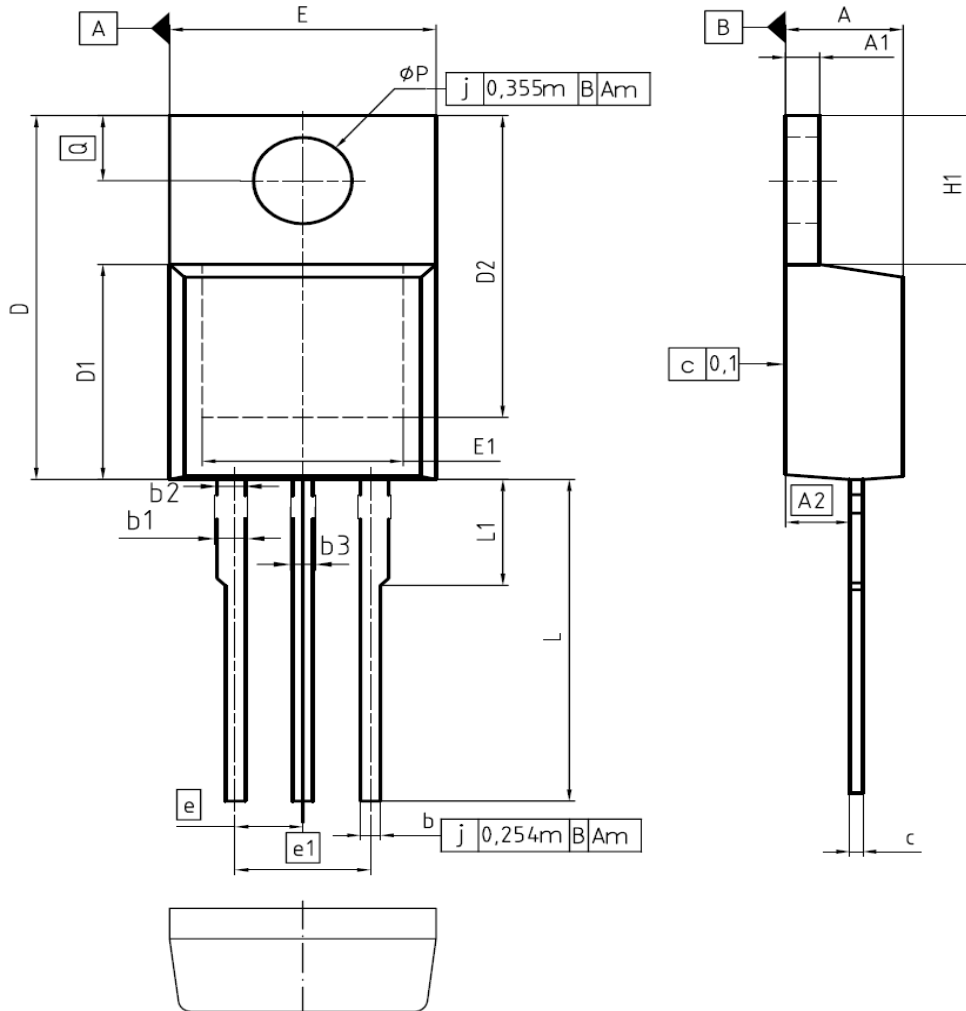
PG-TO220-3-1
