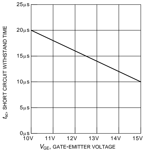
Figure 19. Short circuit withstand time as a function of gate-emitter voltage ( V_{CE} = 600V, \text{start at } T_i = 25^\circ C )
