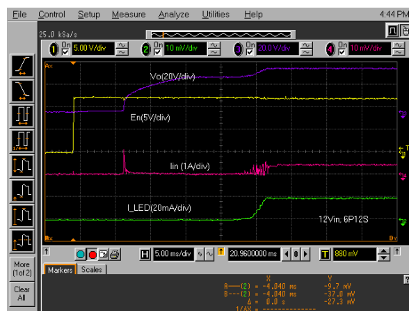
FIGURE 13. IN-RUSH AND LED CURRENT AT V_{IN} = 12V FOR 4P12S AT 20mA/CHANNEL
