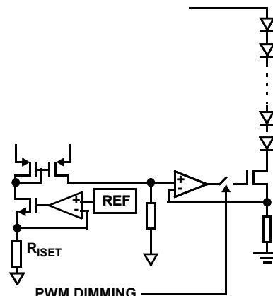
FIGURE 19. SIMPLIFIED CURRENT SOURCE CIRCUIT
