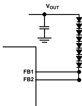
FIGURE 27. GROUPING MULTIPLE CHANNELS FOR HIGH CURRENT APPLICATIONS
