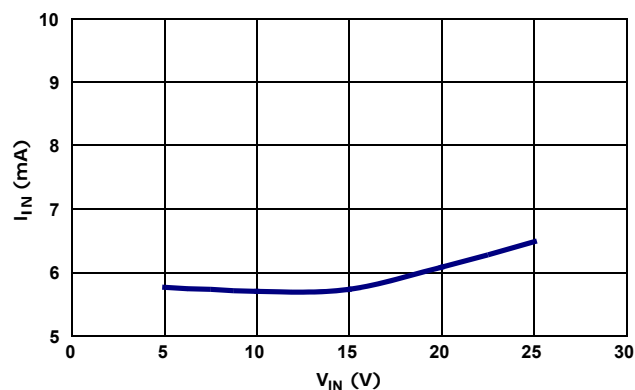
FIGURE 9. QUIESCENT CURRENT vs V_{IN} WITH PART ENABLED
