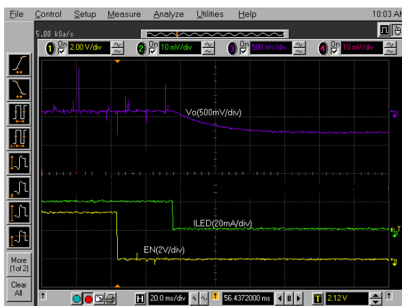
FIGURE 18. ISL97675 SHUTS DOWN AND STOPS SWITCHING ~ 30ms AFTER EN GOES LOW
