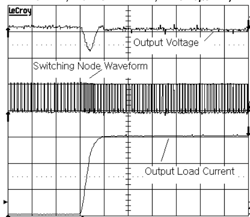
Load Transient Test ( V_{IN}=5V , V_{OUT}=1.2V , I_{OUT}= 0A to 3A , Forced Continuous Conduction Mode, L_{OUT}=1.3μH , C_{OUT}=2x22μF , Channel 1: 50mV/Div, Channel 2: 5V/Div, Channel 4: 1A/Div, Time: 10μs/Div)
