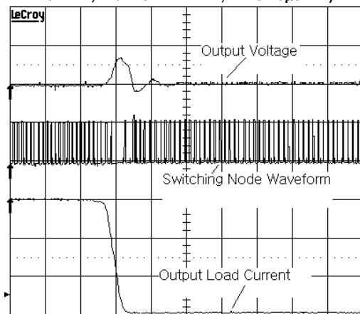
Load Transient Test ( V_{IN}=5V , V_{OUT}=1.2V , I_{OUT}= 3A to 0A , Forced Continuous Conduction Mode, L_{OUT}=1.3μH , C_{OUT}=2x22μF , Channel 1: 100mV/Div, Channel 2: 5V/Div, Channel 4: 1A/Div, Time: 10μs/Div)
