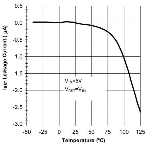
I_{BST} Leakage Current vs Temperature
