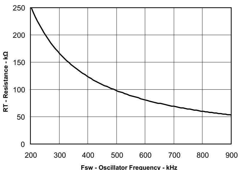
Figure 20. RT Set Resistor vs Switching Frequency
