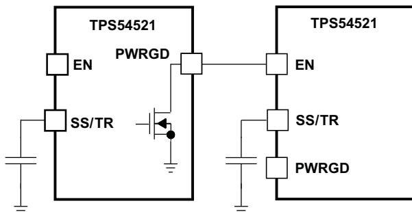
Figure 22. Sequential Start Up Sequence
