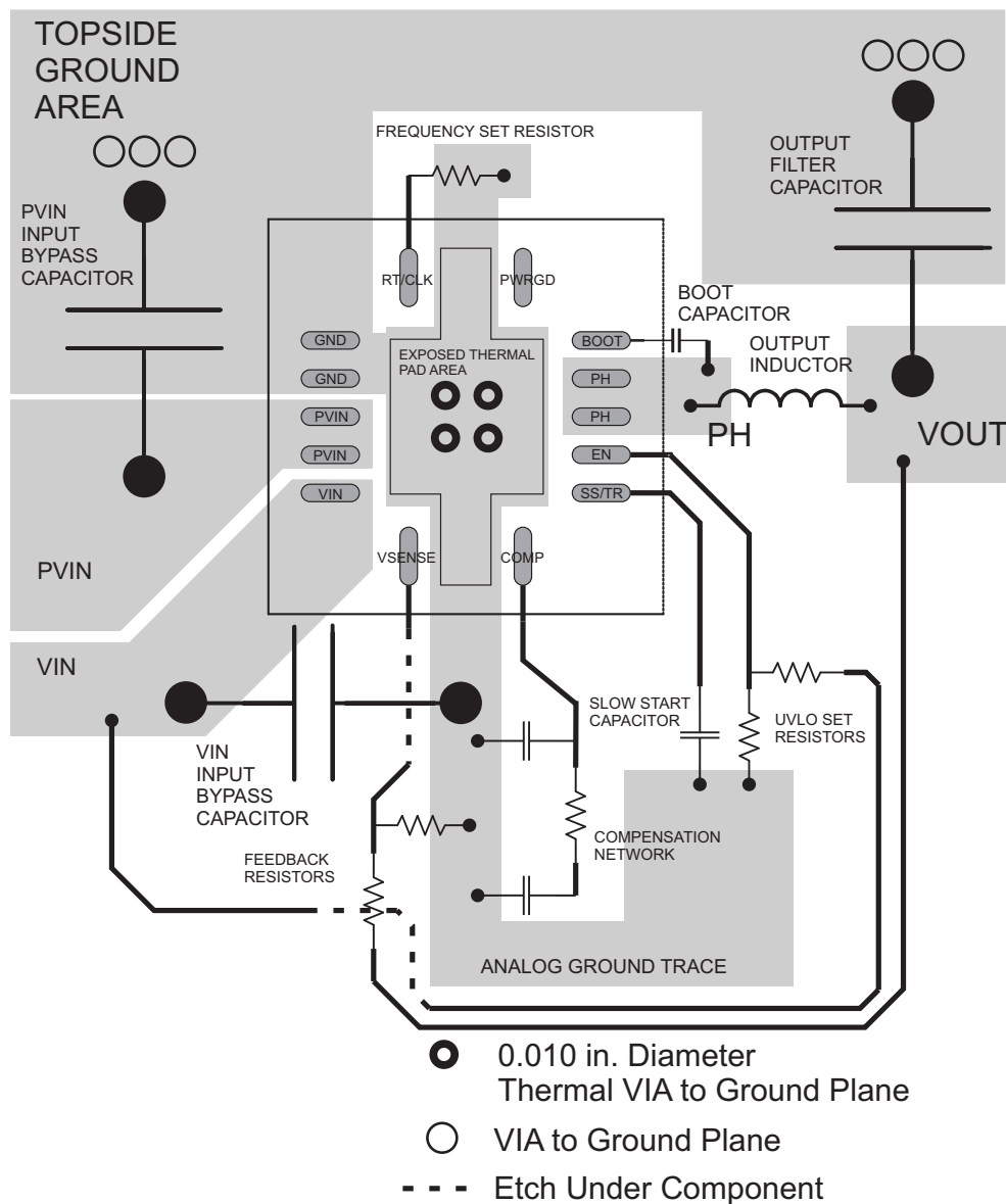
Figure 55. PCB Layout
