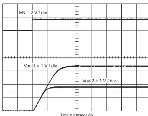
Figure 29. Simultaneous Startup
