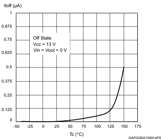
Figure 6. Off-state output current
