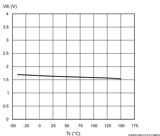
Figure 10. High-level input voltage
