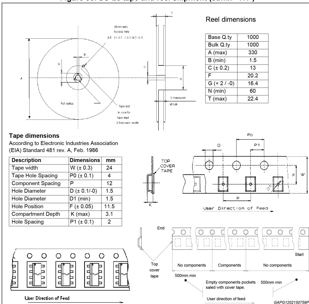
Figure 38. SO-28 tape and reel shipment (suffix "TR")
