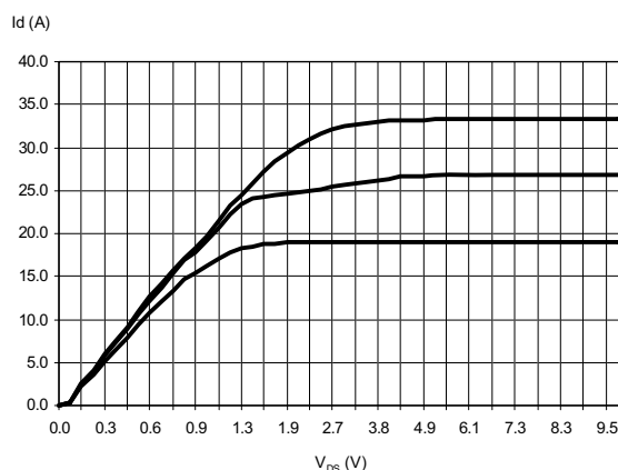
Figure 23. Output characteristics
