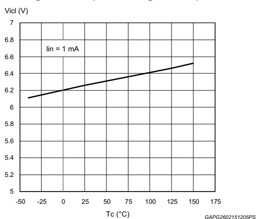
Figure 8. Input voltage clamp
