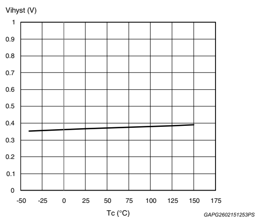
Figure 11. Input voltage hysteresis
