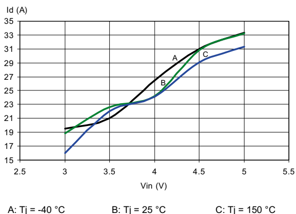
Figure 22. Transfer characteristics
