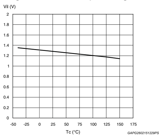
Figure 9. Low level input voltage
