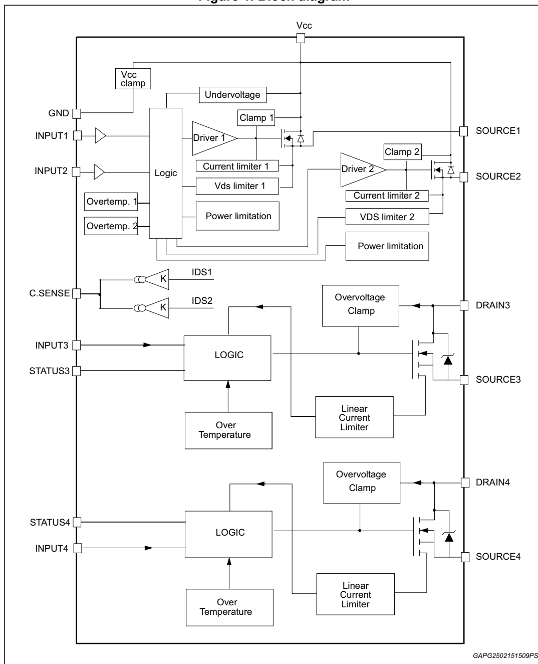
Figure 1. Block diagram
