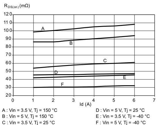
Figure 21. Static drain source on-resistance vs drain current
