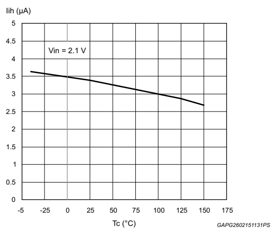
Figure 7. High-level input current
