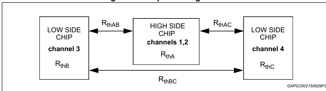
Figure 31. Chipset configuration
