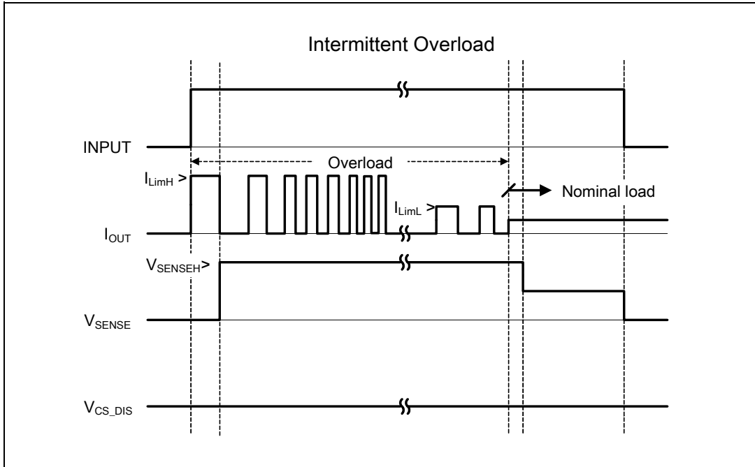
Figure 12. Intermittent overload
