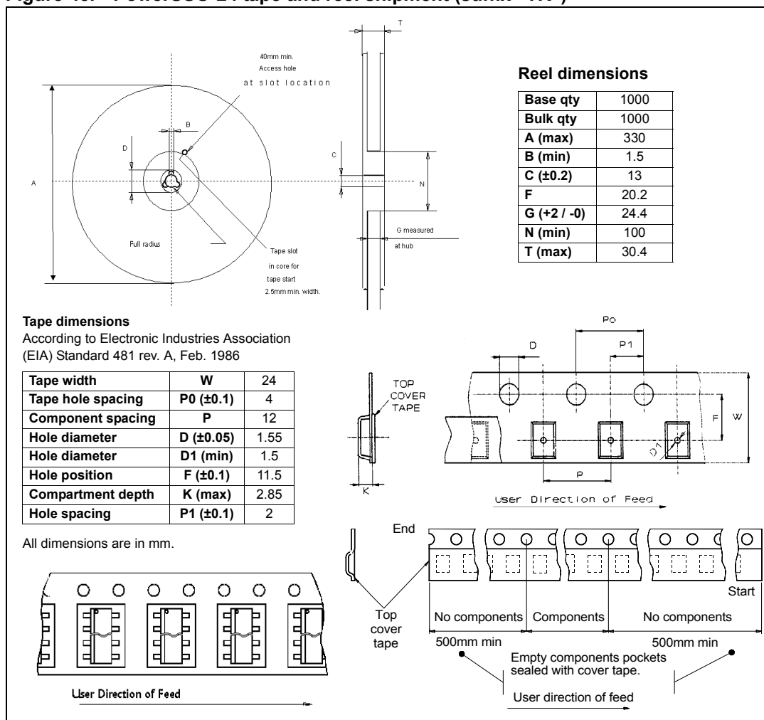
Figure 45. PowerSSO-24 tape and reel shipment (suffix "TR")
