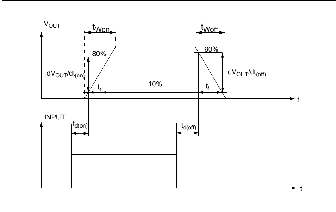
Figure 5. Switching characteristics
