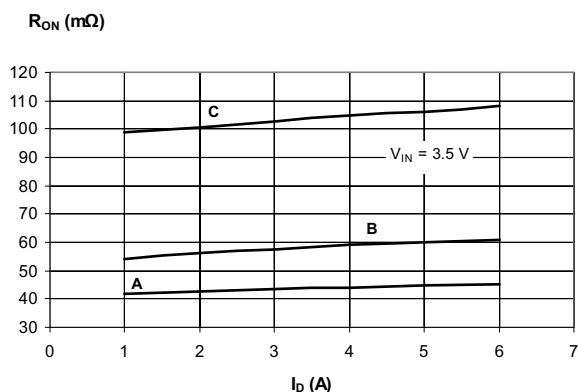
Figure 7. Static drain source on-resistance vs. drain current
