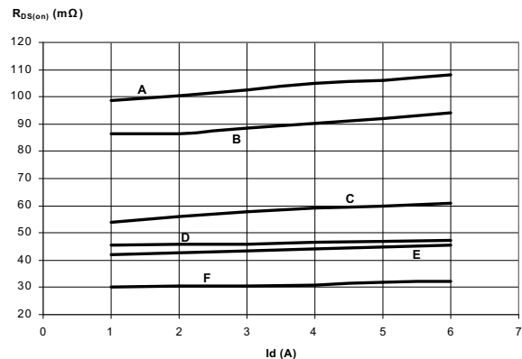
Figure 9. Static drain source on-resistance vs. drain current
