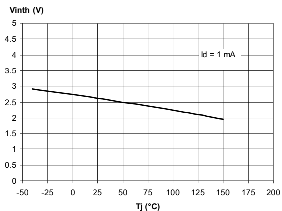
Figure 14. Normalized input threshold vs. temperature
