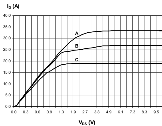
Figure 12. Output characteristics
