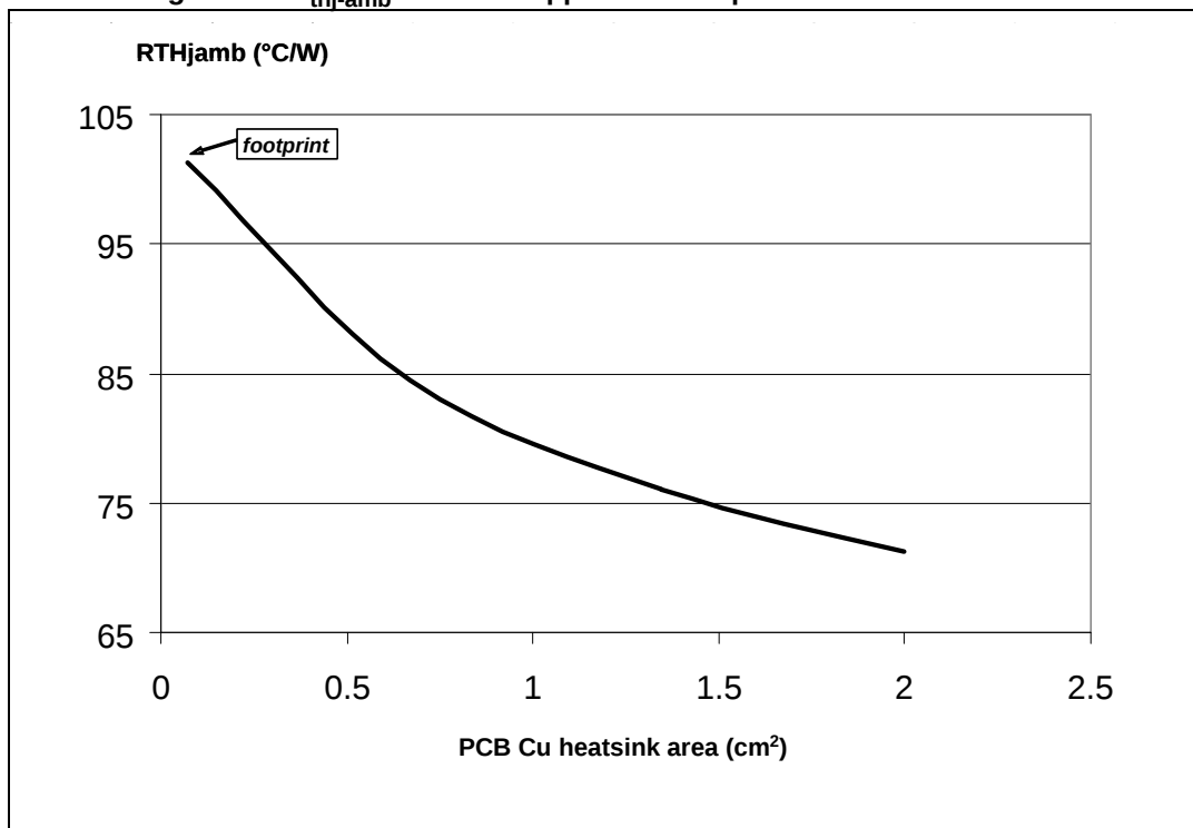
Figure 24. R_{thj-amb} vs. PCB copper area in open box free air condition
