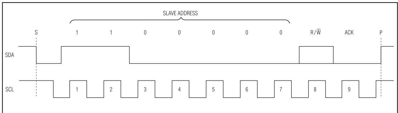
Figure 1. MAX2160 Slave Address Byte
