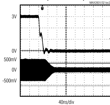
Rx BB VGA SETTLING RESPONSE (-16 GAIN STEP)
