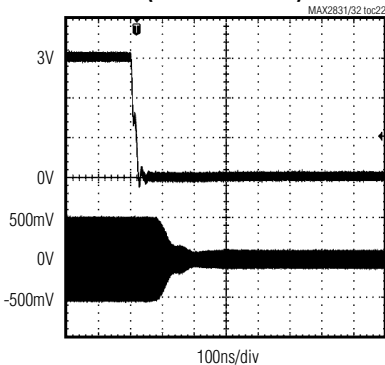
RF LNA SETTLING RESPONSE (HIGH TO MEDIUM)
