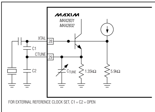
Figure 1. Crystal Oscillator Schematic
