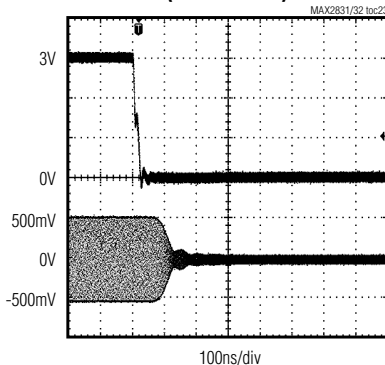
RF LNA SETTLING RESPONSE (HIGH TO LOW)
