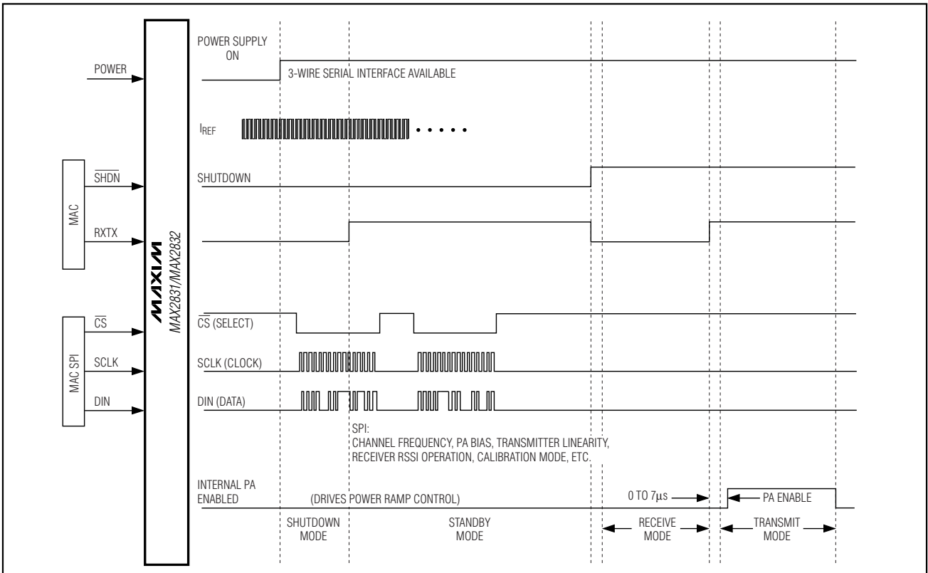
Figure 3. Timing Diagram
