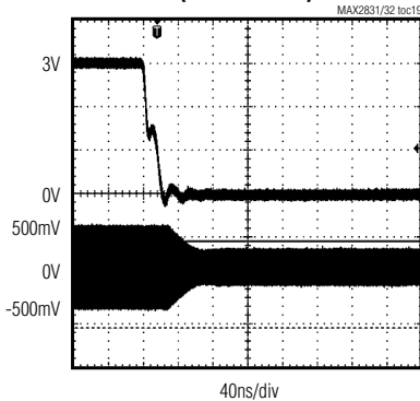
Rx BB VGA SETTLING RESPONSE (-8 GAIN STEP)
