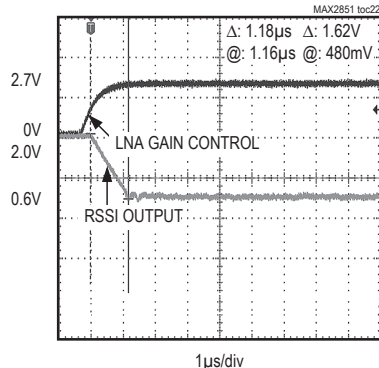
Rx BASEBAND RSSI -32dB STEP RESPONSE
