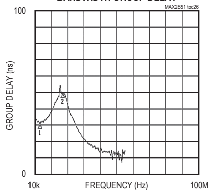
Rx LPF 40MHz CHANNEL BANDWIDTH GROUP DELAY
