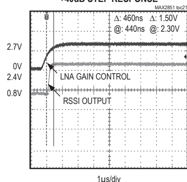
Rx BASEBAND RSSI +40dB STEP RESPONSE
