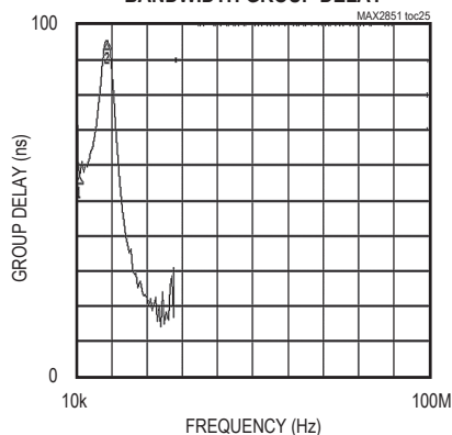
Rx LPF 20MHz CHANNEL BANDWIDTH GROUP DELAY
