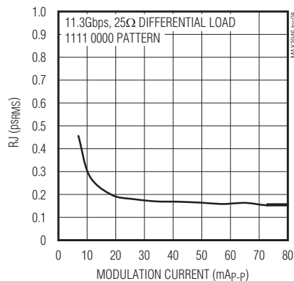
RANDOM JITTER vs. MODULATION CURRENT (AT LOAD)
