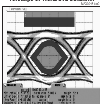
10.3Gbps OPTICAL EYE DIAGRAM
