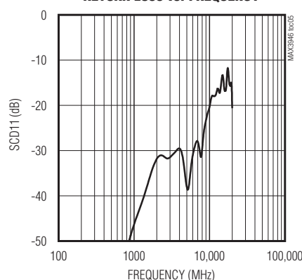
INPUT DIFFERENTIAL TO COMMON-MODE RETURN LOSS vs. FREQUENCY
