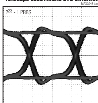
10.3Gbps ELECTRICAL EYE DIAGRAM
