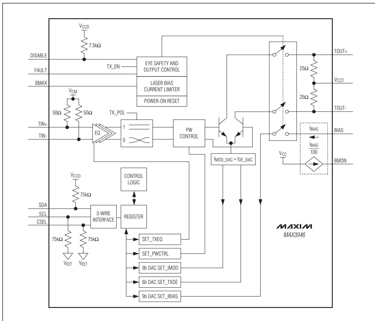
Figure 2. Functional Diagram
