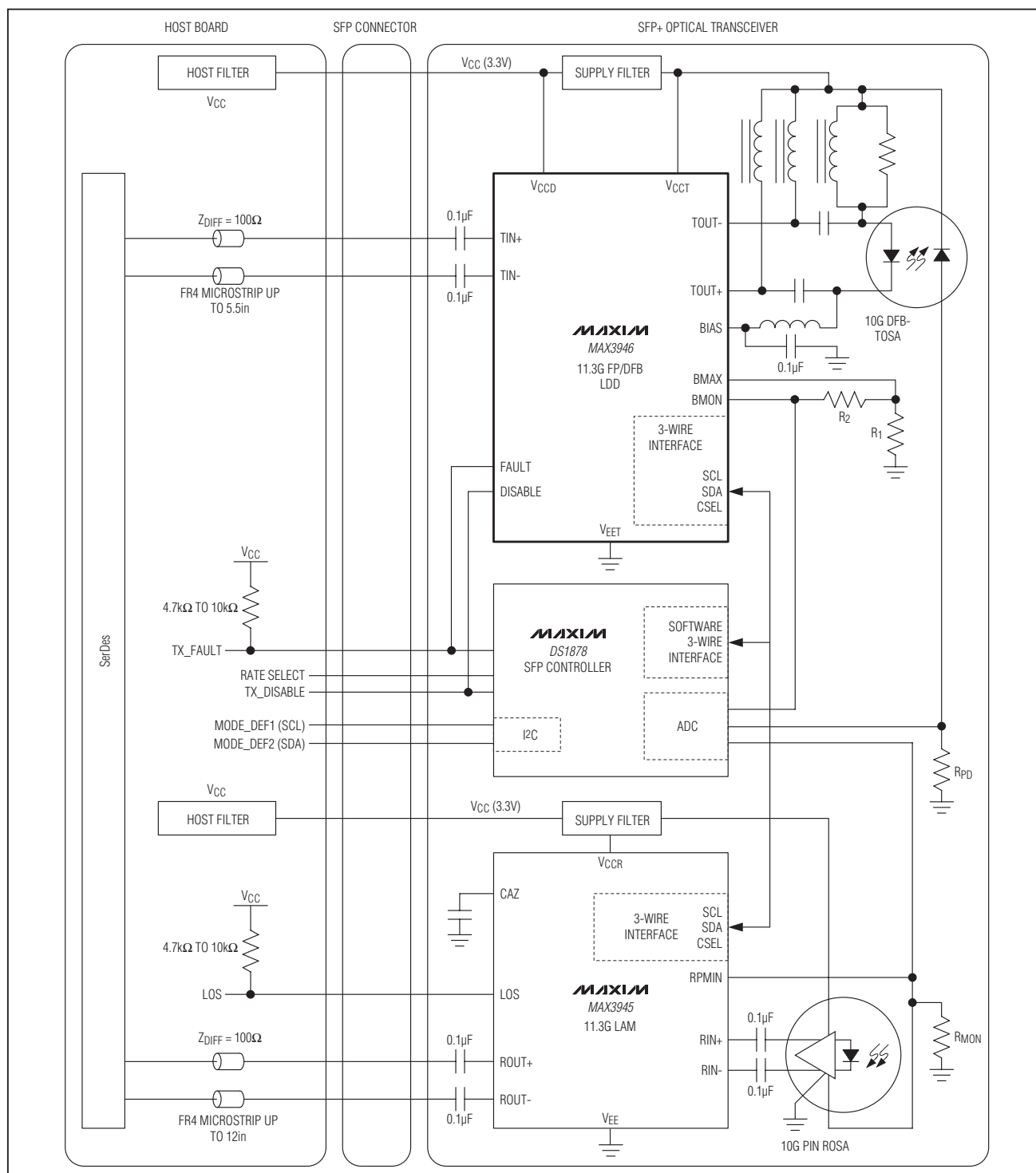
Typical Application Circuit for 10GBASE-LR
