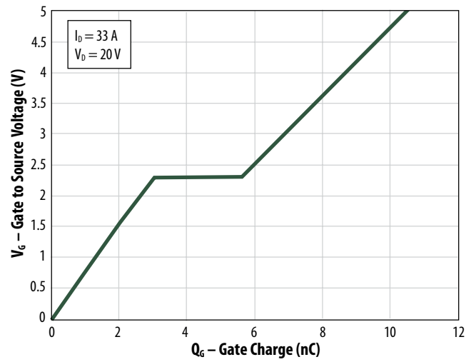
Figure 6: Gate Charge
