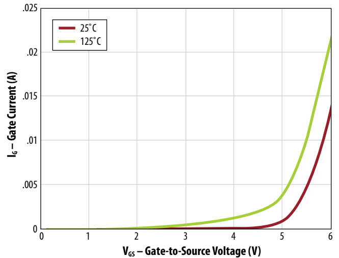
Figure 10: Gate Current
