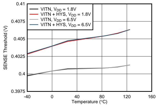
Figure 18. SENSE2 Threshold and Hysteresis vs Temperature
