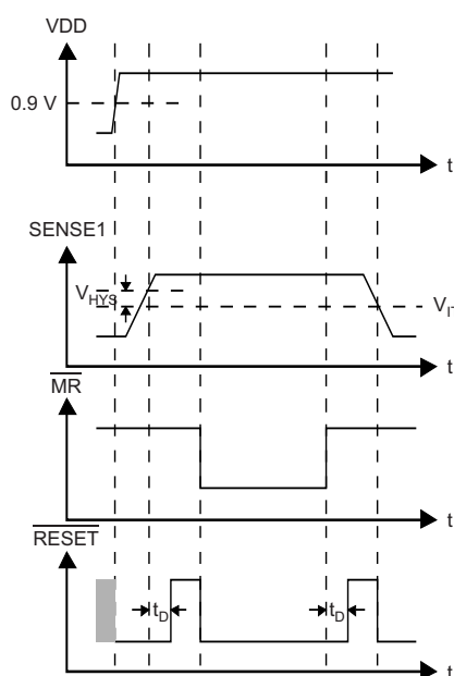
Figure 1. Timing Diagram
