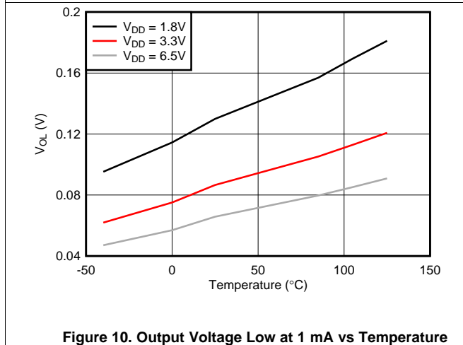
Figure 10. Output Voltage Low at 1 mA vs Temperature
