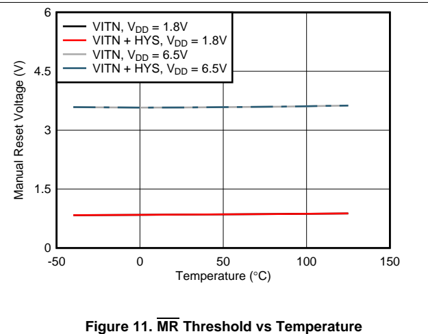
Figure 11. \overline{\text{MR}} Threshold vs Temperature
