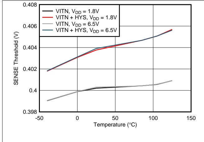
Figure 8. SENSE4 Threshold and Hysteresis vs Temperature
