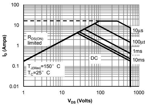
Figure 9: Maximum Forward Biased Safe Operating Area for AOT4N60 (Note F)
