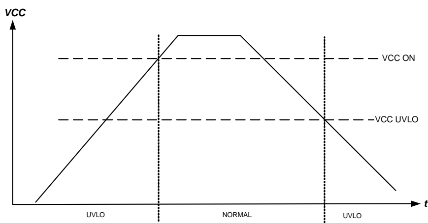
Figure 5: Vcc UVLO
