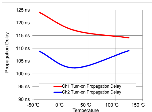
Figure 15: Turn-on Propagation Delay vs. Temperature
