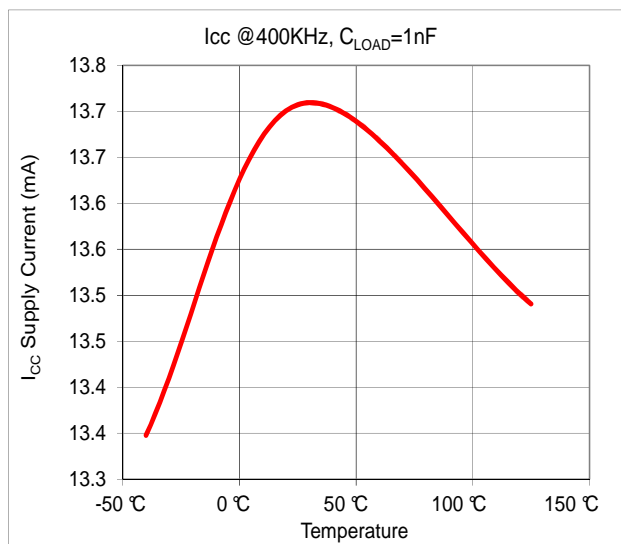
Figure 10: Icc Supply Current @ 1nF Load vs. Temperature
