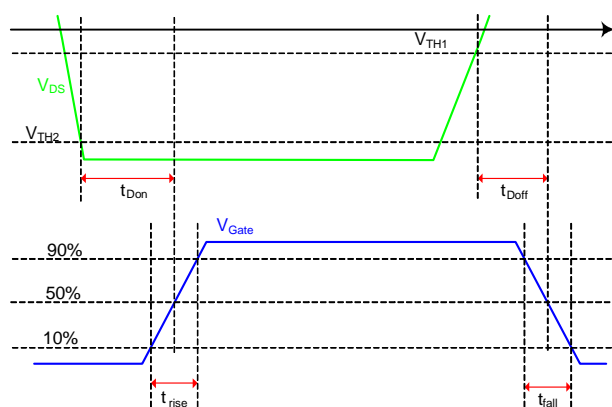
Figure 6: Timing waveform
