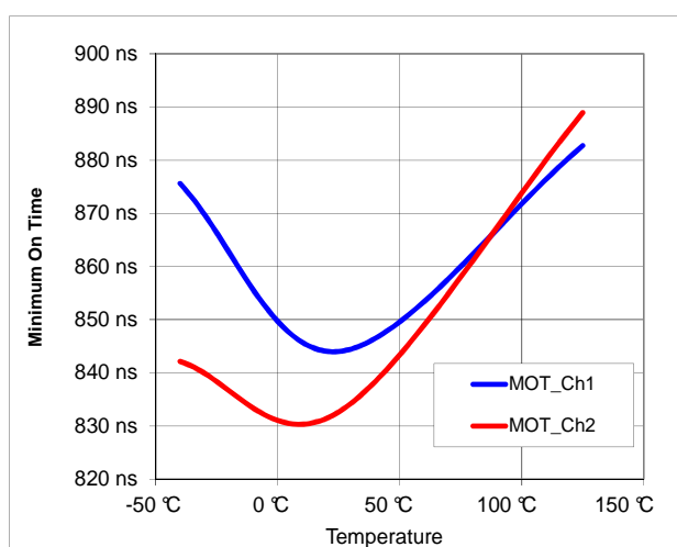
Figure 14: MOT vs Temperature
