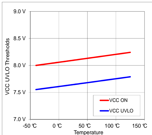
Figure 8: Undervoltage Lockout vs. Temperature
