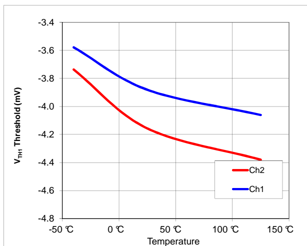
Figure 11: V_{TH1} vs. Temperature
