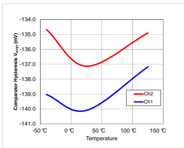
Figure 13: Comparator Hysteresis vs. Temperature
