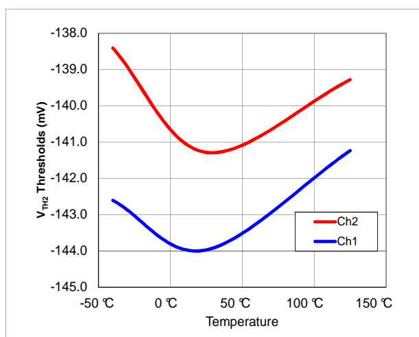
Figure 12: V_{TH2} vs. Temperature
