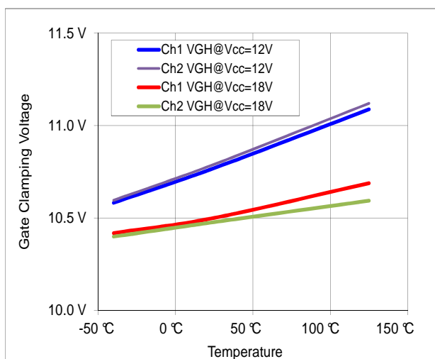
Figure 17: Gate Clamping Voltage vs. Temperature
