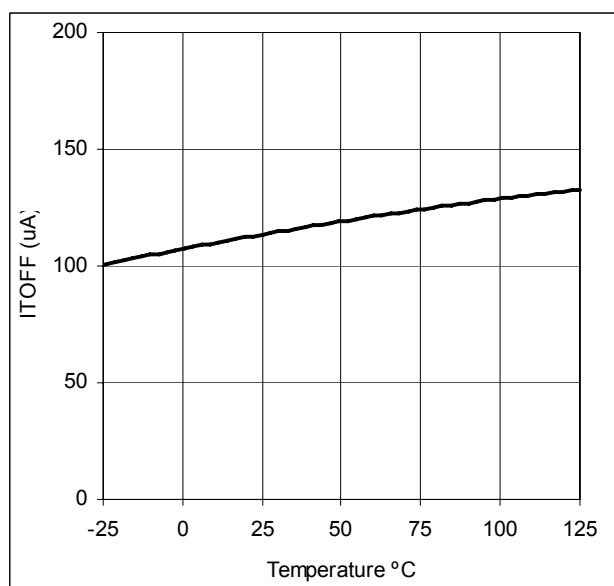
Fig. 17 ITOFF vs. Temperature
