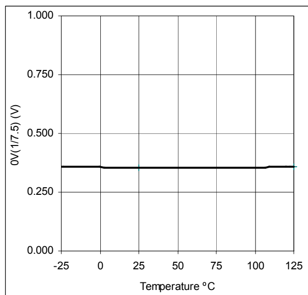
Fig. 16 OV(1/7.5) vs. Temperature
