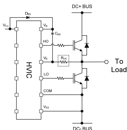
Figure 10: V_S resistor
