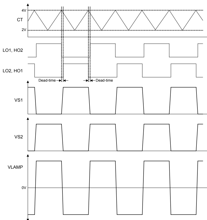
Figure 6, Full-bridge Timing Diagram
