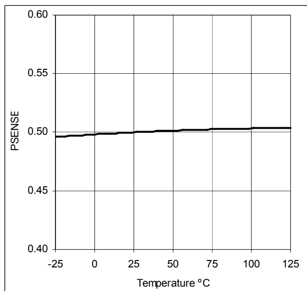
Fig. 13 PSENSE vs. Temperature
