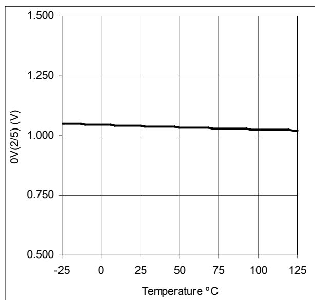
Fig. 15 OV(2/5) vs. Temperature
