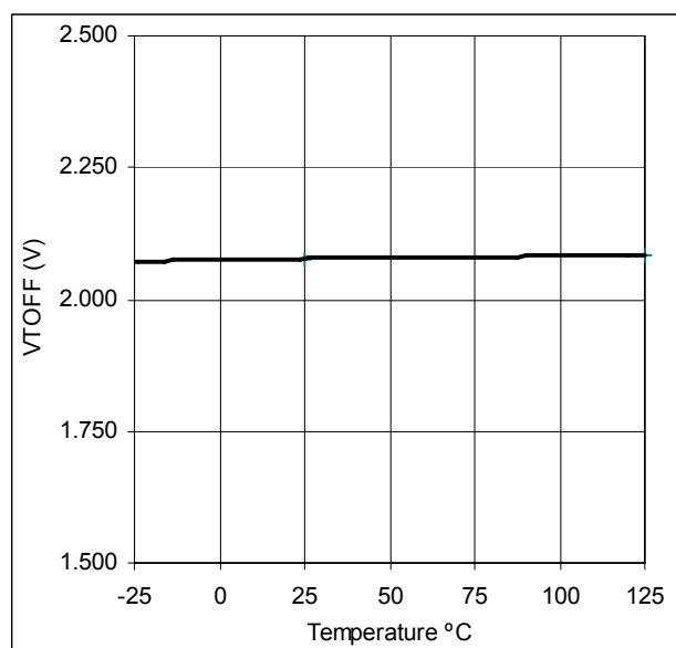
Fig. 18 VTOFF vs. Temperature
