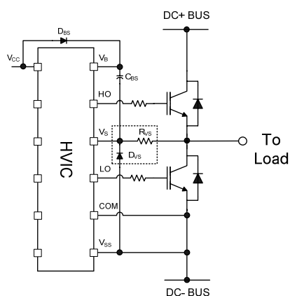
Figure 11: V_S clamping diode
