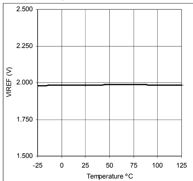
Fig. 11 VIREF vs. Temperature
