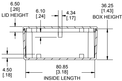
SECTION A-A SIDE VIEW
