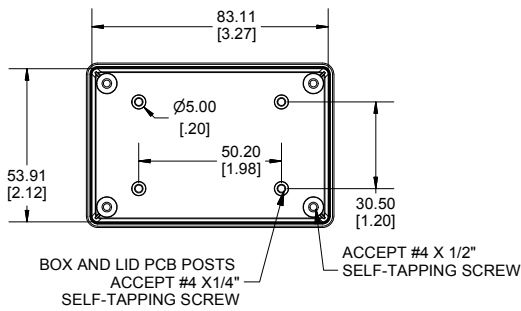
INSIDE BOX
