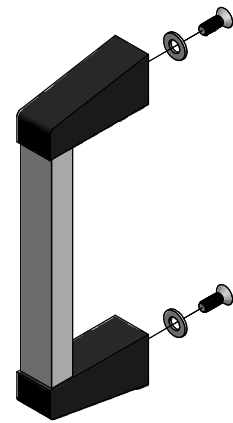
EXPLODED HANDLE ASSEMBLY
