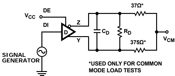
FIGURE 7A. TEST CIRCUIT
