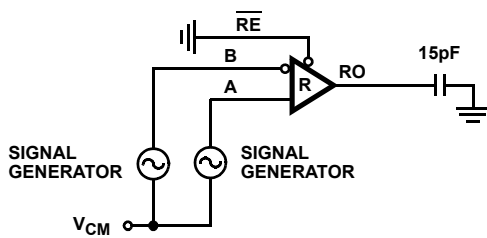
FIGURE 10A. TEST CIRCUIT
