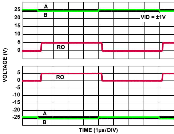
FIGURE 24. ±25V RECEIVER PERFORMANCE (ISL31490E, ISL31491E, ISL31492E)
