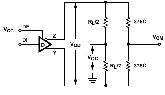
FIGURE 6B. V_{OD} AND V_{OC} WITH COMMON MODE LOAD
