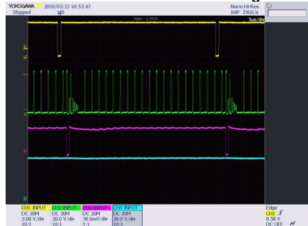
Ch 1 (yellow) – PWM signal at 30 kHz 98% duty cycle C2 (green) – SW node voltage, Ch 3(red) – LED Current. Ch4 (blue) - V_{OUT}
