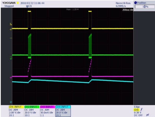
Ch 1 (yellow) – PWM signal at 1 kHz 5% duty cycle C2 (green) – SW node voltage, Ch 3(red) – LED Current. Ch4 (blue) - V_{OUT}
