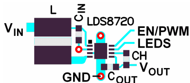
Figure 3. Recommended layout
