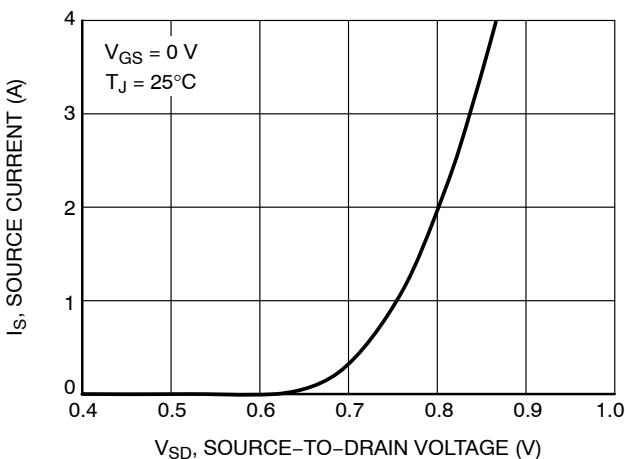
Figure 11. Diode Forward Voltage vs. Current
