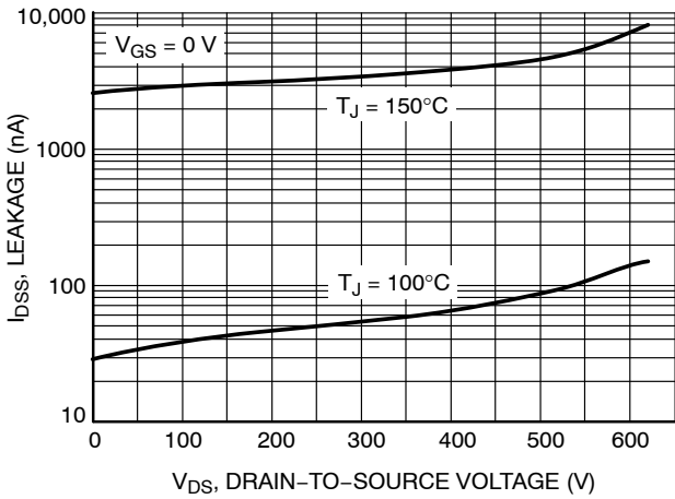
Figure 7. Drain-to-Source Leakage Current vs. Voltage
