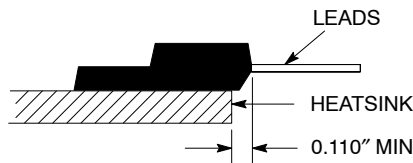
Figure 14. Isolation Test Diagram
