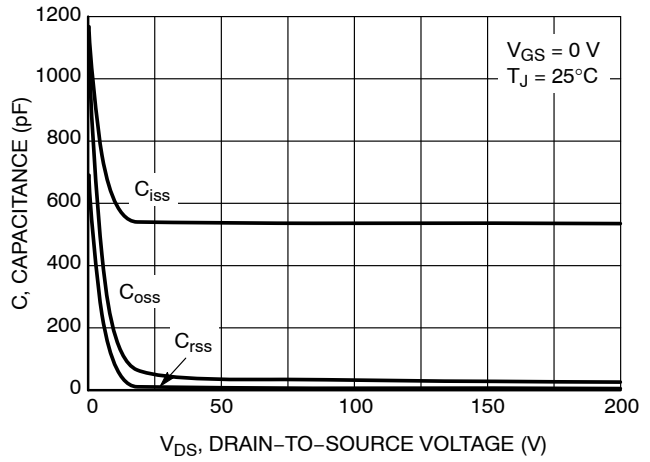
Figure 8. Capacitance Variation
