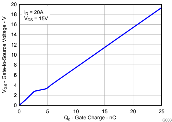
Figure 4. Gate Charge
