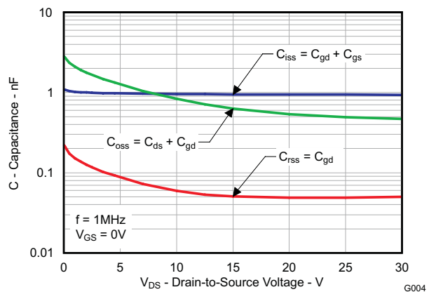
Figure 5. Capacitance
