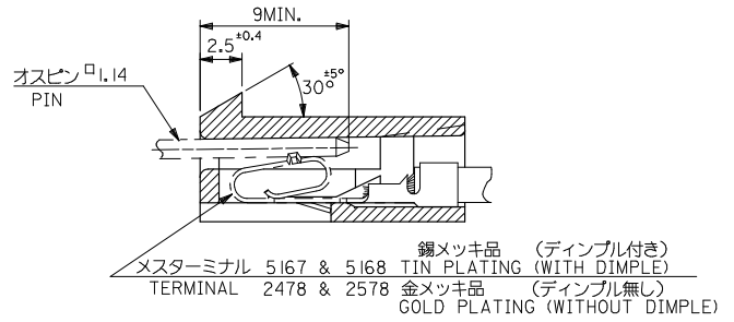
SECT. C-C
