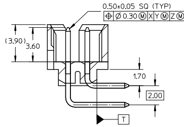
SECTION Y-Y
