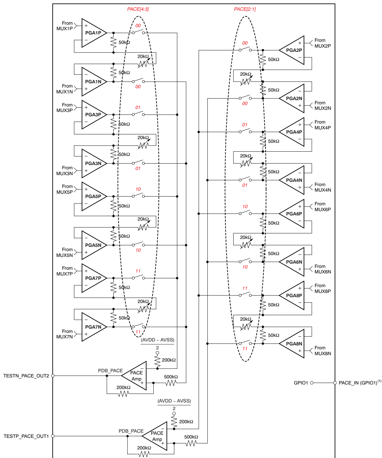
Figure 53. Hardware Pace Detection Option
