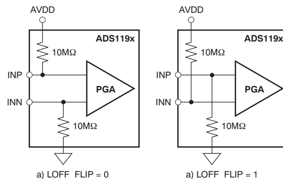
Figure 48. LOFF_FLIP Usage
