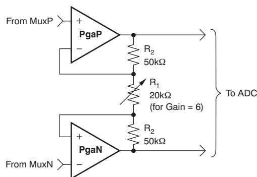
Figure 19. PGA Implementation
