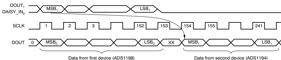
Figure 37. Daisy-Chain Timing
