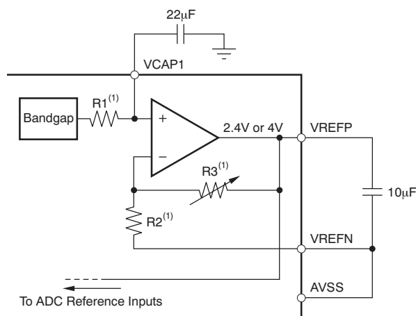
Figure 26. Internal Reference
