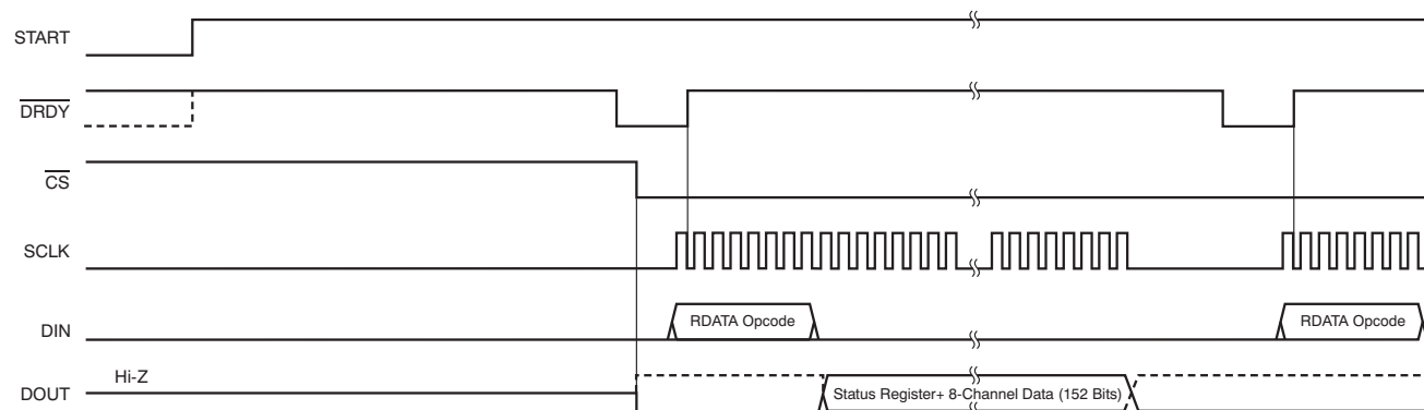
Figure 39. RDATA Usage
