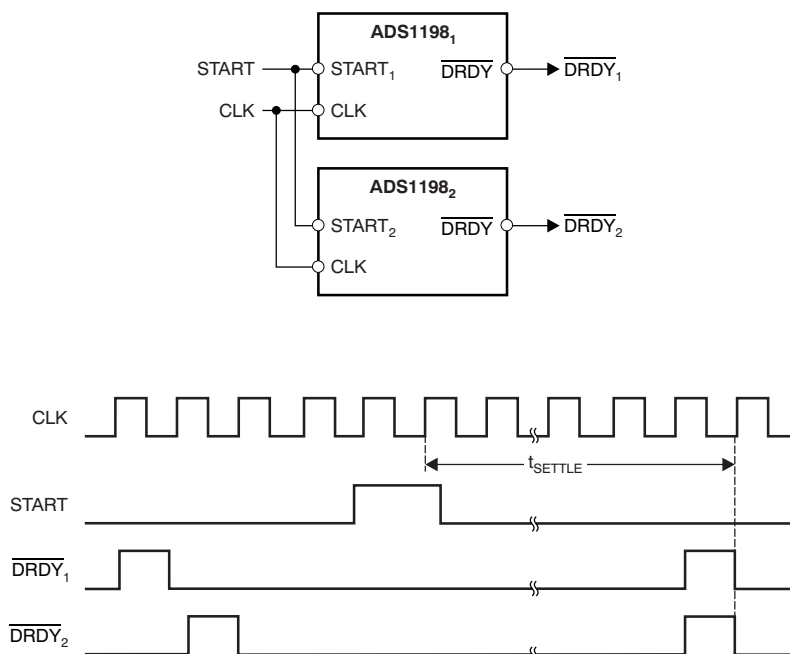
Figure 35. Synchronizing Multiple Converters
