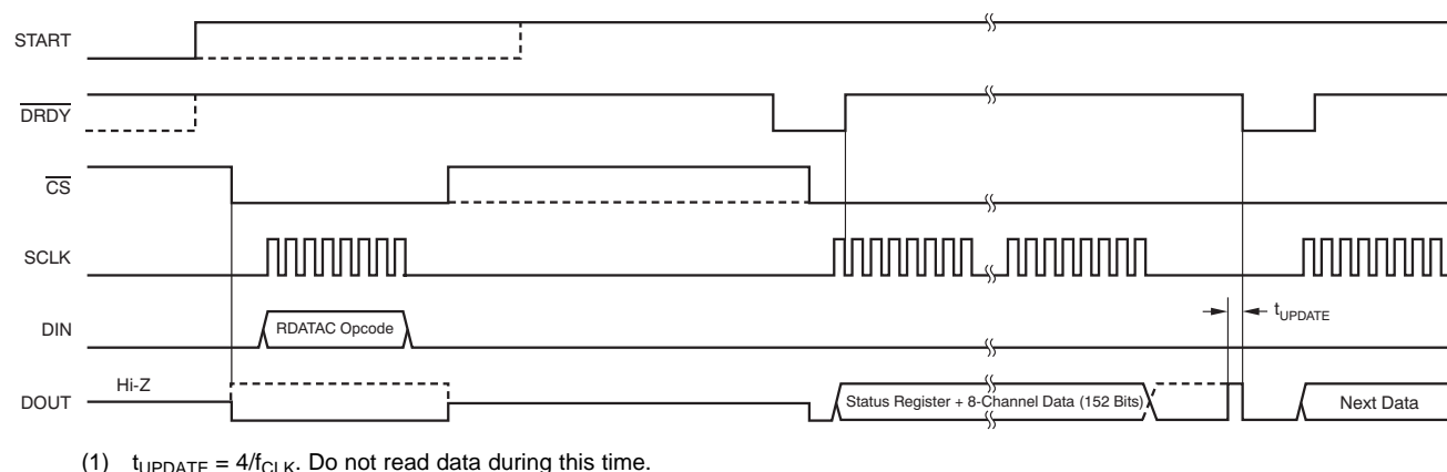
Figure 38. RDATAC Usage
