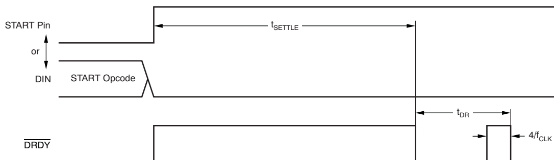
Figure 31. Settling Time
