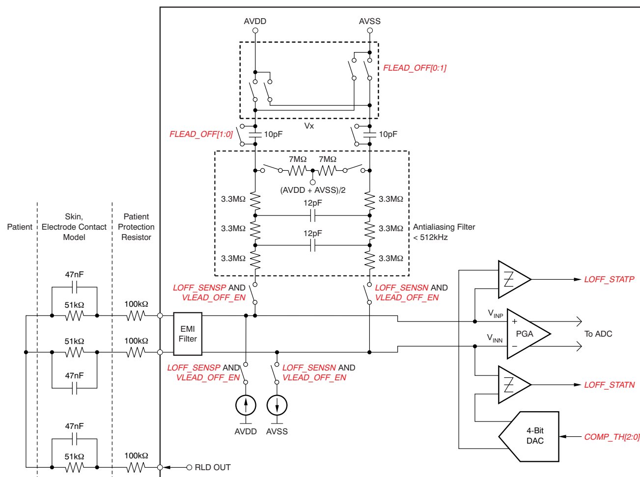
Figure 46. Lead-Off Detection
