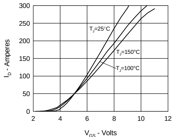
Fig. 2 Input Admittance
