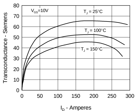
Fig. 6 Transconductance
