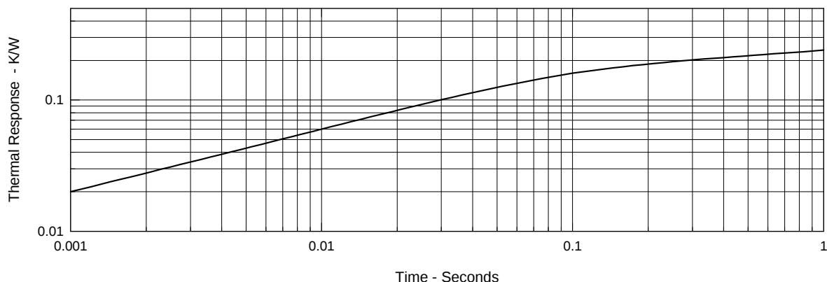
Fig.10 Transient Thermal Impedance
