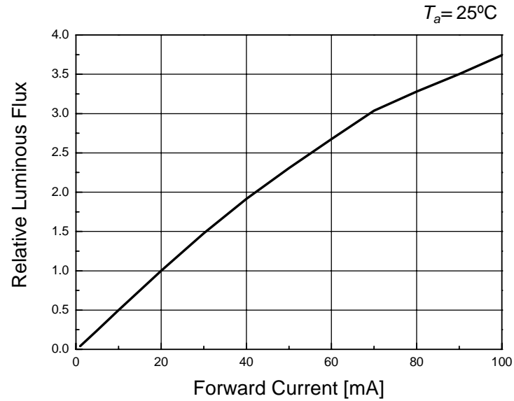
Forward Current vs. Relative Intensity
