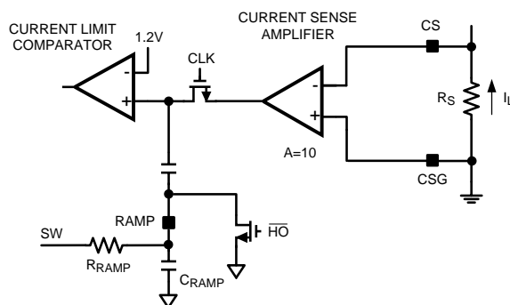
Figure 10. Current Limit and Ramp Circuit
