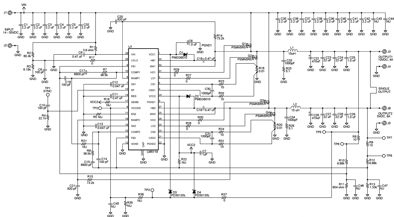
Figure 14. 10-V 4-A, 5-V 8-A Typical Application Schematic
