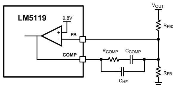
Figure 16. Feedback Configuration
