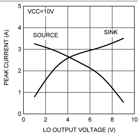
Figure 2. LO Peak Driver Current vs Output Voltage
