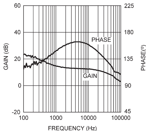
Figure 19. Error Amplifier Gain and Phase
