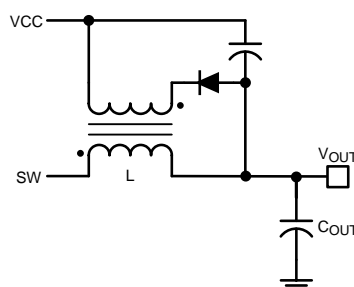
Figure 8. VCC Bias Supply With Additional Inductor Winding
