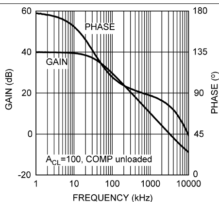
Figure 7. Error Amp Gain and Phase vs Frequency
