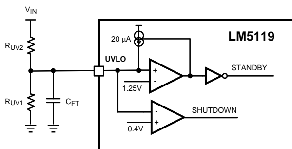
Figure 17. UVLO Configuration
