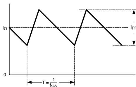
Figure 15. Inductor Current
