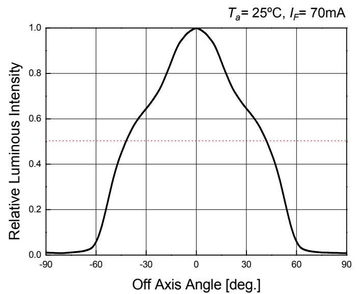
Directivity
