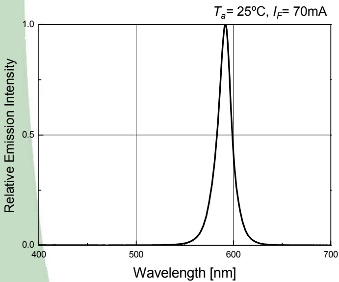
Spectrum
