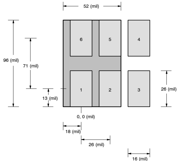
FIGURE 2. SC-70 (6 leads) Single
