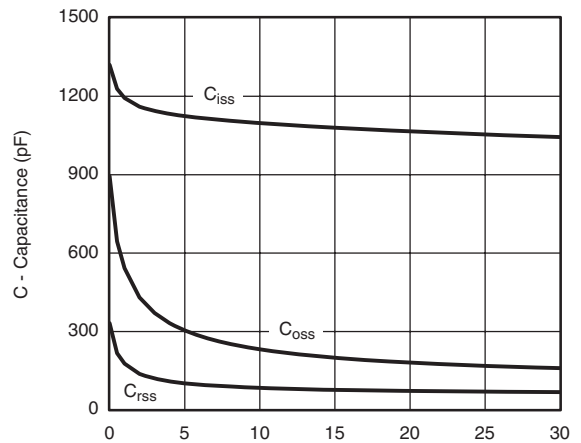
Capacitance
