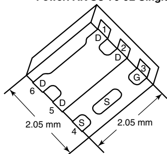
PowerPAK SC-70-6L-Single
