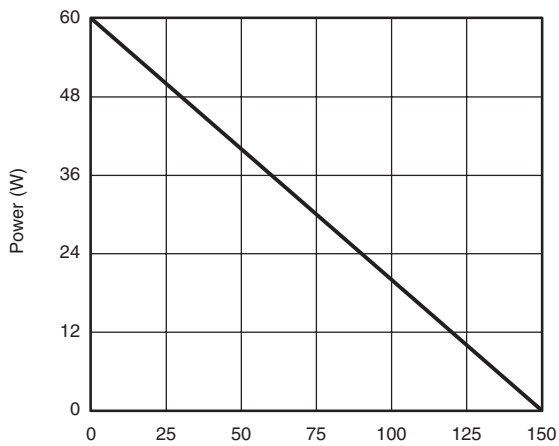
Power, Junction-to-Case
