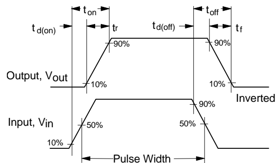
Figure 12. Switching Waveforms
