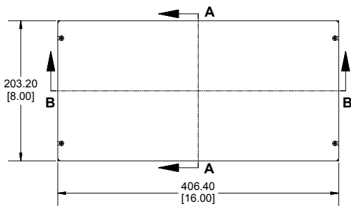
Bottom View of Assembly
