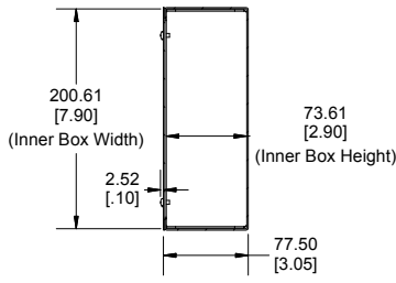
SECTION A-A End View of Assembly
