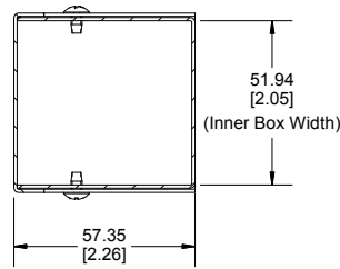
SECTION A-A End View of Assembly
