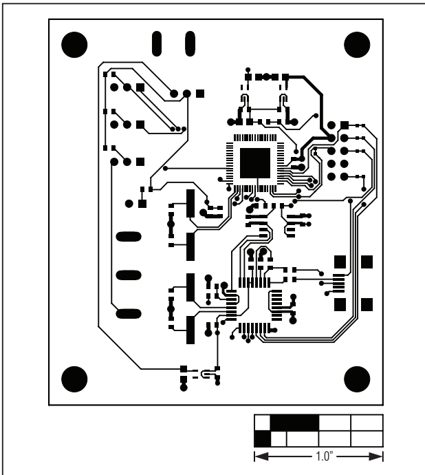
Figure 6. MAX9635 EV Kit PCB Layout—Solder Side
