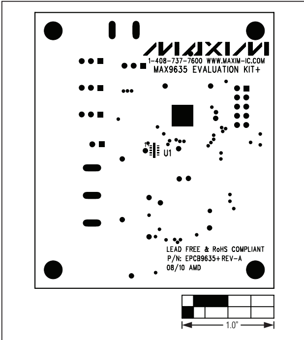
Figure 4. MAX9635 EV Kit Component Placement Guide—Component Side
