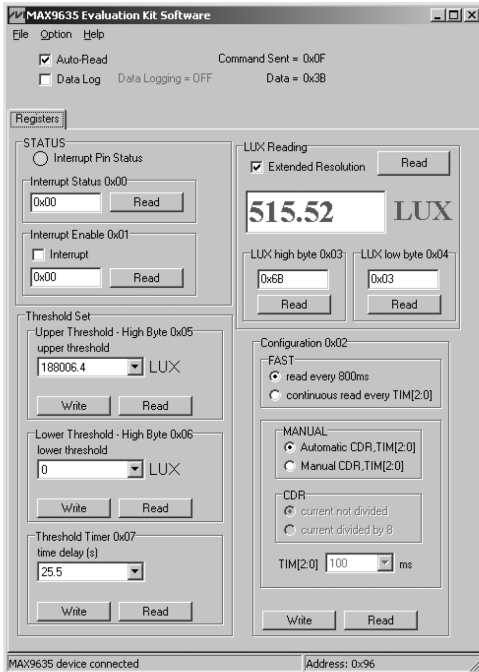
Figure 1. MAX9635 EV Kit Software Main Window
