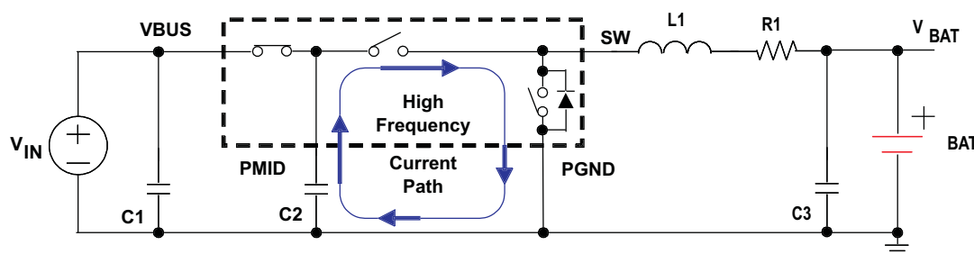
Figure 39. High Frequency Current Path
