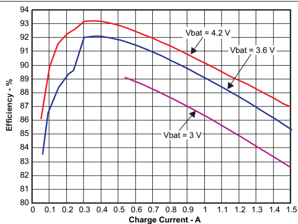
Figure 7. Charger Efficiency
