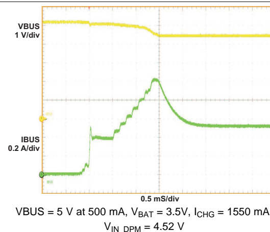
Figure 4. Charge Current Ramp Up
