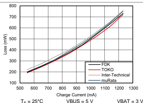
Figure 27. Measured Battery Charge Loss
