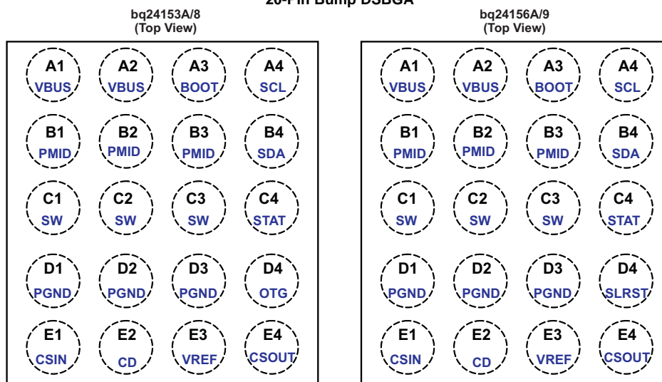
YFF Package 20-Pin Bump DSBGA
