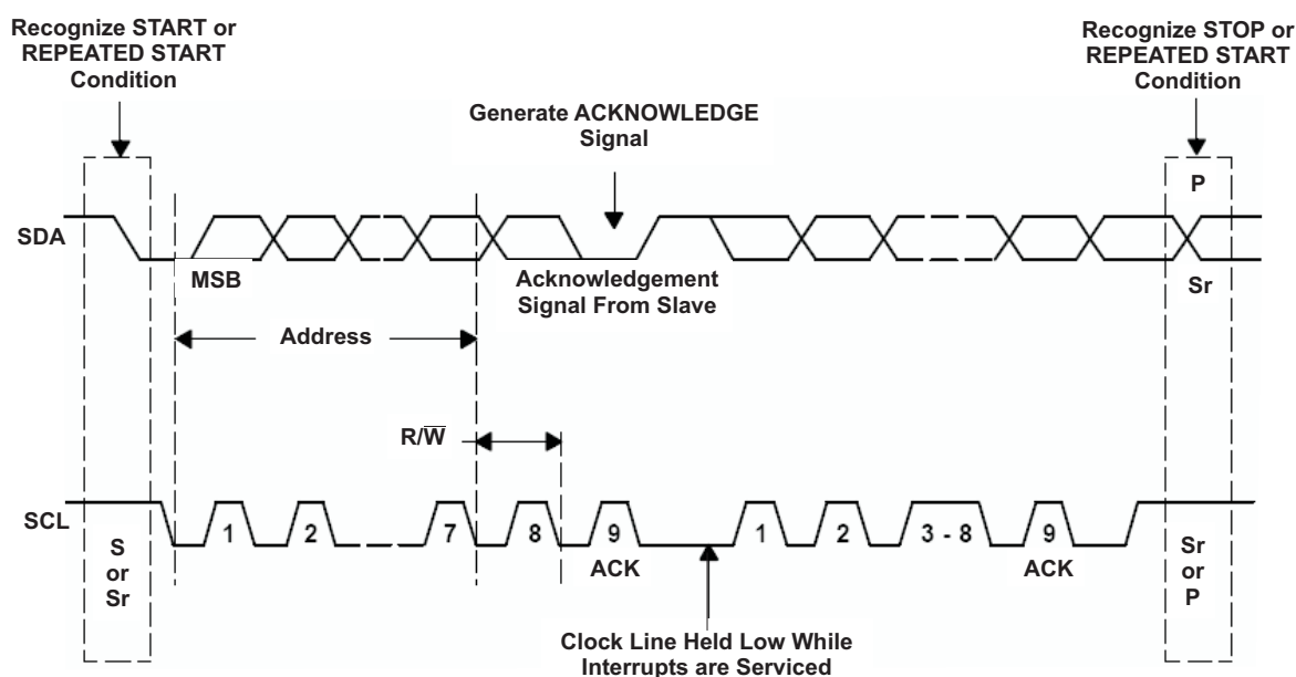
Figure 23. Bus Protocol
