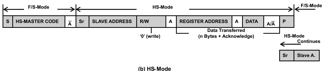
Figure 24. Data Transfer Format in F/S Mode and H/S Mode
