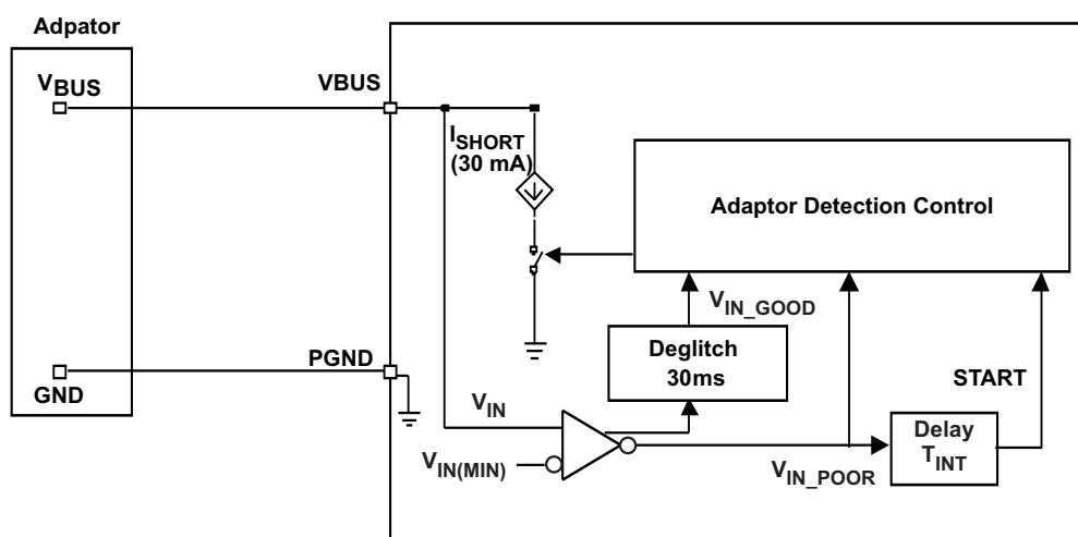
Figure 15. Bad Adaptor Detection Circuit
