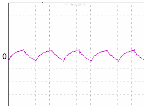
Figure 14: Output voltage ripple at nominal input voltage and rated load current ( I_o=40A )(100 mV/div, 1µs/div) Load capacitance: 1µF ceramic capacitor and 10µF tantalum capacitor. Bandwidth: 20 MHz. Scope measurements should be made using a BNC cable (length shorter than 20 inches). Position the load between 51 mm to 76 mm (2 inches to 3 inches) from the module.
