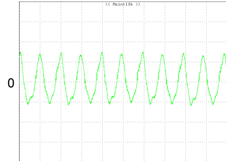
Figure 11: Input Terminal Ripple Current, i_c , at full rated output current and nominal input voltage with 12µH source impedance and 100µF electrolytic capacitor (100 mA/div, 2µs/div)
